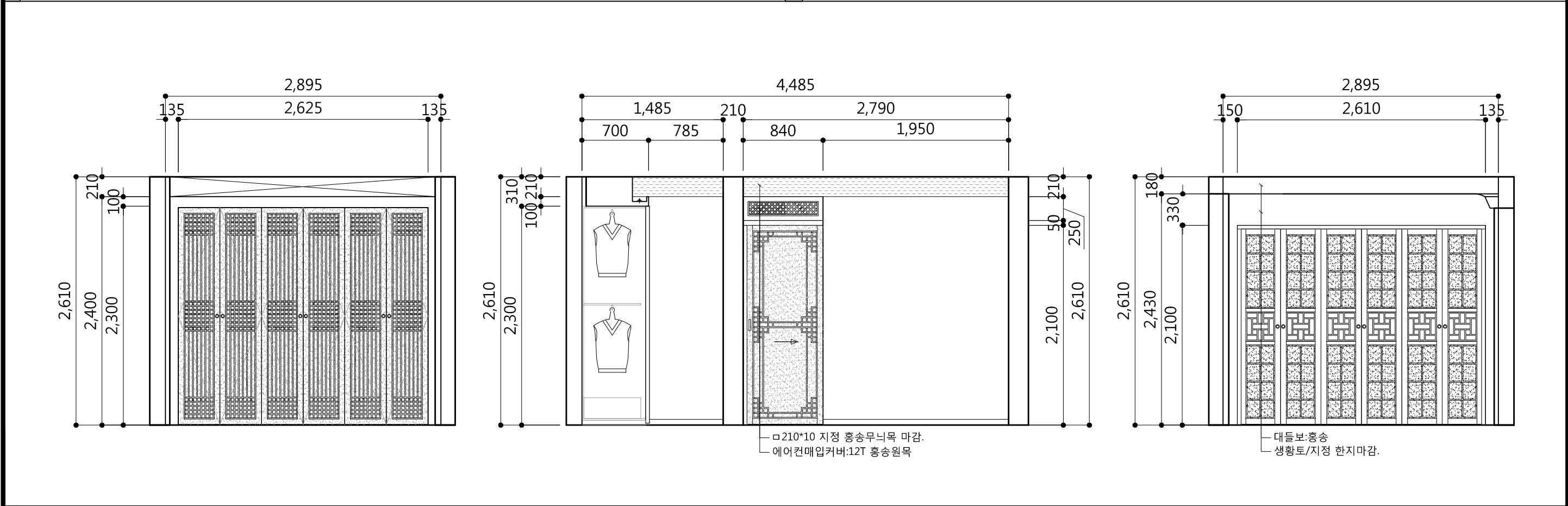
3 전통형 안방 ELEVATION B,C,D SCALE-A3:1/40, A4:1/60
